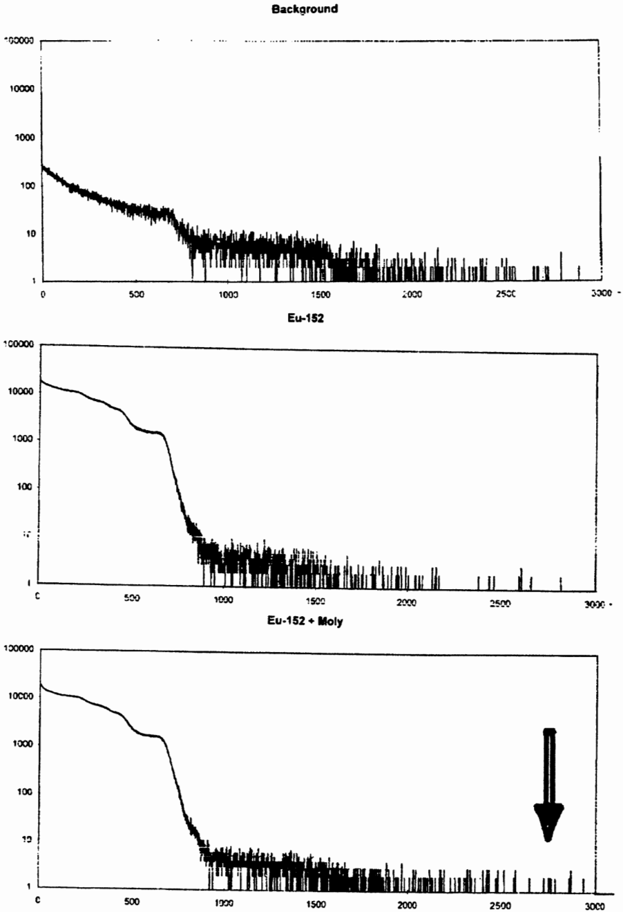
Figure 7.38. A view of the detection by Tsagas for the background, the Europa isotope alone, and the Europa-Molybdenum paid (below) showing the detection of emission over 1 MeV that can solely be of nuclear origin, thus confirming, although in a preliminary way, Santilli prediction [87].
