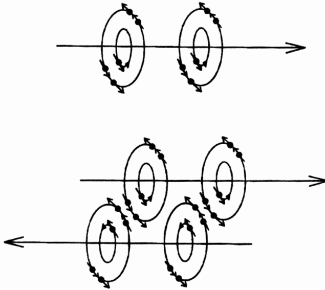
Figure 7.16. A schematic view of the singlet (antiparallel) spin coupling necessary to synthesize the helium from deuterium according to nuclear synthesis (7.38) which is of evident very difficult engineering realization for controlled systematic fusions.
