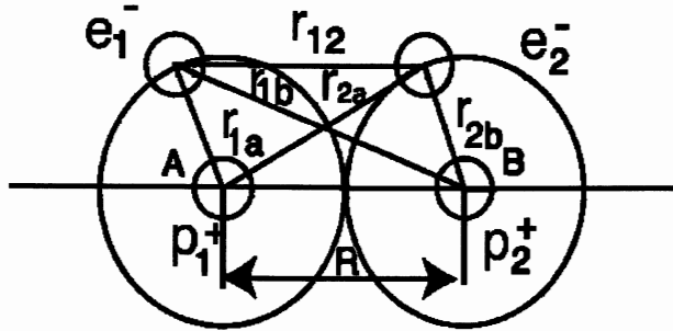
Figure 4.5. A view of all possible conventional interactions between the two electrons and the two protons of a hydrogen molecules. Being quantum mechanical, all these interactions are solely at a distance derivable from a potential, as in Eq. (4.12), thus being basically insufficient for a representation of the short term nonpotential interactions in valence bonds.
