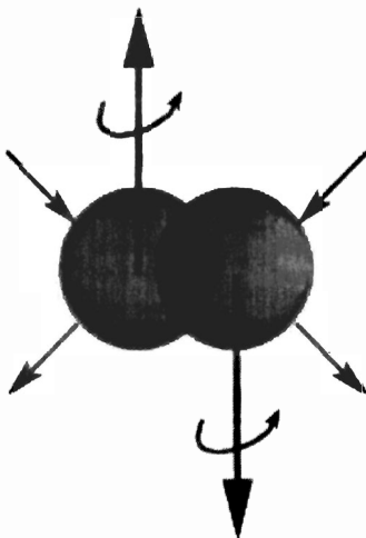
Figure 1.4. The new interactions at the foundations of hadronic mechanics originating from mutual contact and penetration of the wavepackets of particles at short distances that are non-Hamiltonian because nonlinear, nonlocal and nonpotential, thus requiring a nonunitary lifting of quantum mechanics, including its mathematics, physical laws and experimental verifications.
