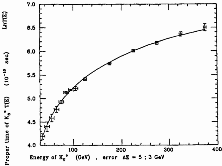
Figure 5.5. The exact plot done by Cardone et al. (loc. cit.) of the seemingly divergent experimental data of both Aronson's and Grossman's experimental data (loc. cit.) via Santilli's isometric in the energy range from 30 to 400 GeV. These plots provided an experimental confirmation of Santilli's isolaw (5.18) in the interior of kaons with numerical values (5.29)–(5.39). Note the clear emergence of a deviation from the Einsteinian law (5.16) despite its (claimed) recovering by Grossman's measurements. The experiments here considered are manifestly fundamental because they establish deviations from the Minkowskian spacetime in the interior of hadrons in favor of Minkowski-Santilli isospacetime due to its direct universality. In turn, the generalization of the basic geometry within hadronic matter has far reaching implications in particle physics, nuclear physics, astrophysics and other fields, including new clean energies. As shown in subsequent chapters, the tests here considered also signal the initiation of a new technology based, for the first time, on strong interactions, an occurrence simply impossible under the exact validity of special relativity in the interior of hadrons.
