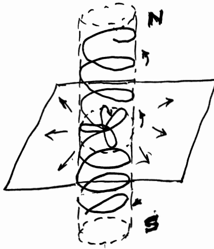
Figure 3.3. An original drawing by Santilli dating back to 1955 on his conception of the origin of the magnetic field of the electron conceived as a pure oscillation of space, showing the clear duality of the field along the rotational symmetry axis originating from deformations of space perpendicular to the characteristic structural oscillation.
