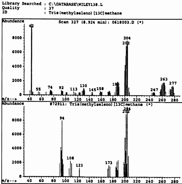
Figure 4.13. Following the identification of the unexpected peaks in the mass spectrum of the preceding figure, the analysts requested the computers of the Air Force Basis (containing in excess of 500,000 molecules) to identify the individual peaks. Contrary to expectation, the computer failed to produce the identification of any of the peaks of the preceding scan. Hence, the analysts indicated to Santilli that he had apparently produced "new yet unknown molecules."
