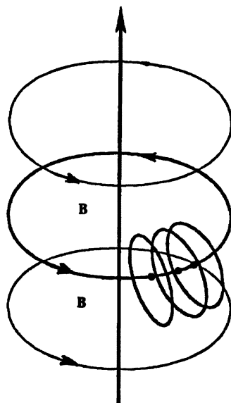
Figure 7.8. A schematic view of the geometry of a DC electric arc represented by the vertical line with the associated magnetic field represented by horizontal circles, and the created magnecules represented by circles perpendicular to the magnetic lines. This geometry has the following primary implications: 1) Since the magnetic field M is proportional to I/r , one can see that at atomic distances from electric arcs with one thousand Amperes of current, the magnetic field is of the order of 10^{11} Gauss, thus being sufficient to polarize atomic orbitals into toroids, and then coupling them into magnecules.
