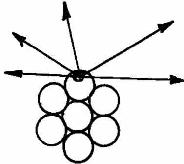
Figure 6.12. Reproduction of a drawing used by Santilli to illustrate that the variation of the kinetic energy in nuclear beta decay is due to the Coulomb interaction between the positively charged nuclei and the negatively charged electron, being maximal for radial emission and minimal for tangential emissions. This results in the well known bell-shaped behavior of the kinetic energy of the emitted electron with no energy at all to permit the very existence of the neutrino.
