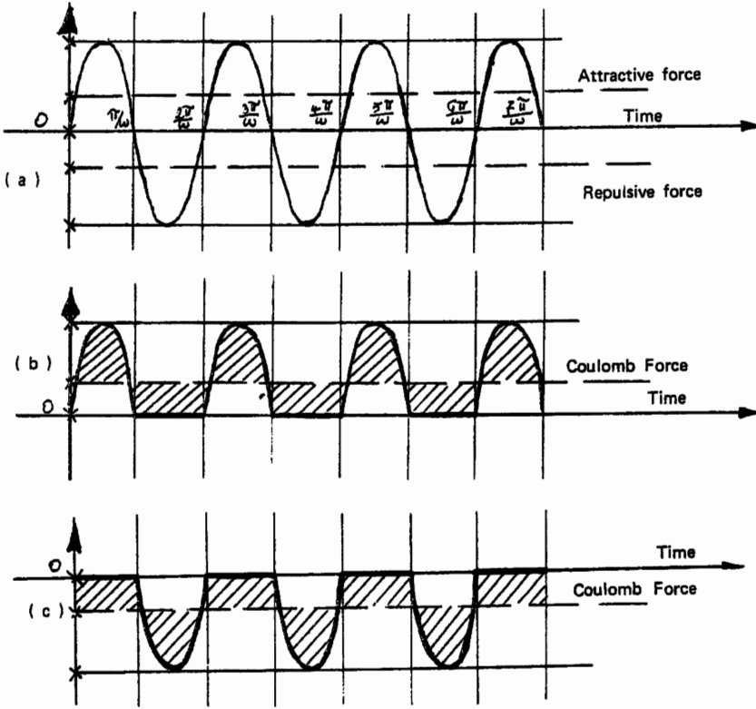
Figure 3.2. Another original drawing by Santilli dating back to 1955 on his conception of the elementary charge of the electron according to Eq. (3.2) as containing both attractive and repulsive actions (top view), which actions are separated into repulsive or attractive force when coupling elementary charges of the same or opposite sign, respectively (lower views).
