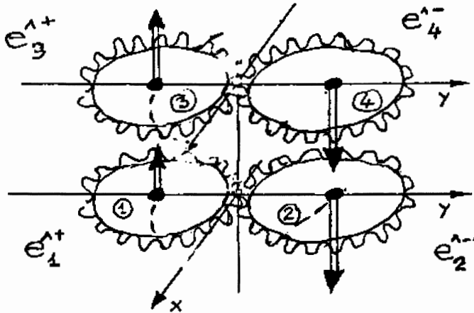
Figure 6.7. Reproduction of the original figure of memoir 1978B to illustrate the structure model of the \eta meson with four elementary massive constituents. Note the “compression” of two \hat{\pi}^0 one inside the other.
