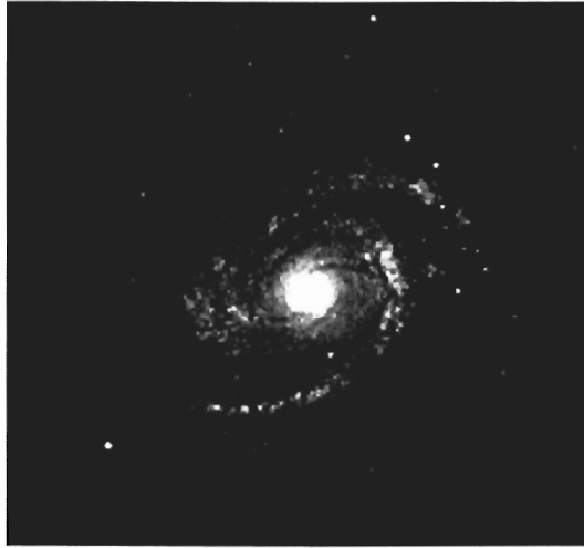
Figure 5.24. The 20th century astrophysics and cosmology assumed that interstellar space inside a given galaxy is empty so as to verify special relativity. Santilli (2007) pointed out that space within a galaxy is filled up with matter whose density decreases with the radial distance from the galactic center, thus causing a slowdown of the speed of light that decreases with the increase of said distance, by eliminating altogether the need for dark matter.
