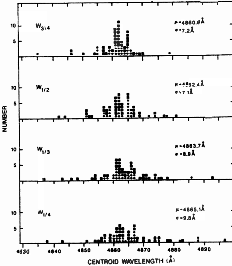
Figure 5.29. The numerical, exact and invariant fit of the experimental data by Sulentic on the quasars internal blue- and red-shifts done by Santilli via the use of isorelativity. The above interpretation is prohibited by the validity of special relativity within physical media, because the “universal constancy of the speed of light” prohibits a frequency dependence that is specific for locally varying speeds. In different words, isorelativity essentially reduces the quasars internal red- and blue-shifts to Newton spectral decomposition of light.
