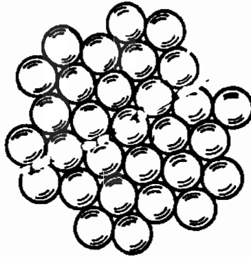
Figure 6.24. A view often used by Santilli to illustrate that nuclei are composed by extended constituents in contact with each other, thus prohibiting that the nuclear force is solely of potential type because the latter solely applies for action-at-a-distance forces among point-like particles. The need for a nonpotential component in the nuclear force motivated the birth and construction of hadronic mechanics.
