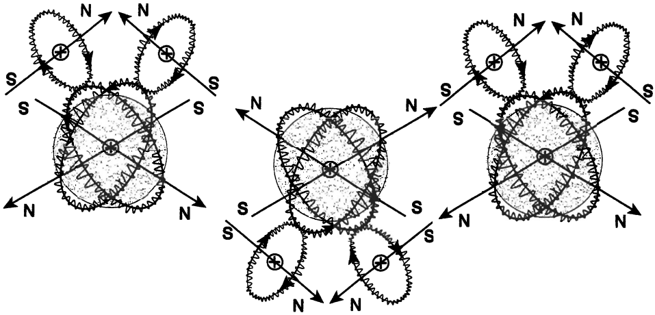
Figure 4.21. A schematic view of the magnecular structure of the liquid state of water discovered by Santilli and presented in FHC. The magnecular structure can be confirmed via a mere inspection of the presence of magnetic fields in the natural state of the water molecule as in Figure 4.7, whose coupling via opposing polarities North-South-North-South results precisely in the magnecular structure of this figure.
