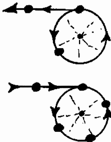
Figure 6.13. Reproduction of the original drawing made and used by Santilli to illustrate the absence of a neutrino in both the neutron synthesis and its decay. In the neutron synthesis in the core of a star (bottom view) the linear momentum of the electron is constrained to be turned into its angular momentum when compressed inside the proton. In the spontaneous decay of the neutron, we have the opposite event in which the constrained angular momentum is transformed into the linear momentum of the expelled electron, its spin being not mutated in first nonrelativistic approximation in both cases.
