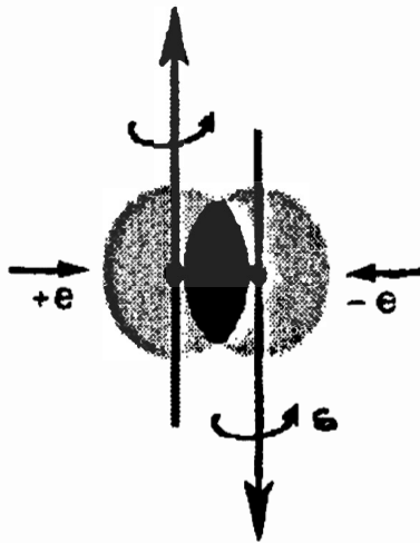
Figure 6.2. A schematic view of the main interactions absent in the structure of the hydrogen atom, but present in the neutron synthesis of Figure 6.1, the nonlinear, nonlocal and nonpotential interactions due to deep wave overlapping of extended particles. Their non-Hamiltonian character mandates a nonunitary covering of quantum mechanics. This motivated the birth of hadronic mechanics in Spring 1978.
