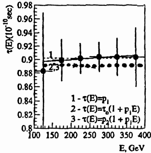
Figure 5.7. A plot of the same data as those of Figure 5.6 run by Santilli in HMMC Volume IV via the use of d parameters different than those used by Aronson et al. showing the extremely unsettled character of claimed “experimental results” when obtained via the use of ad hoc parameters and functions fit from the experimental data within the context of established doctrines. In fact, Santilli’s plot shown in this figure obtained via the use of the same experimental data as those used by Aronson et al. show clear deviations from special relativity expected in any case for an irreversible decay process due to the strict reversibility of the assumed theory.
