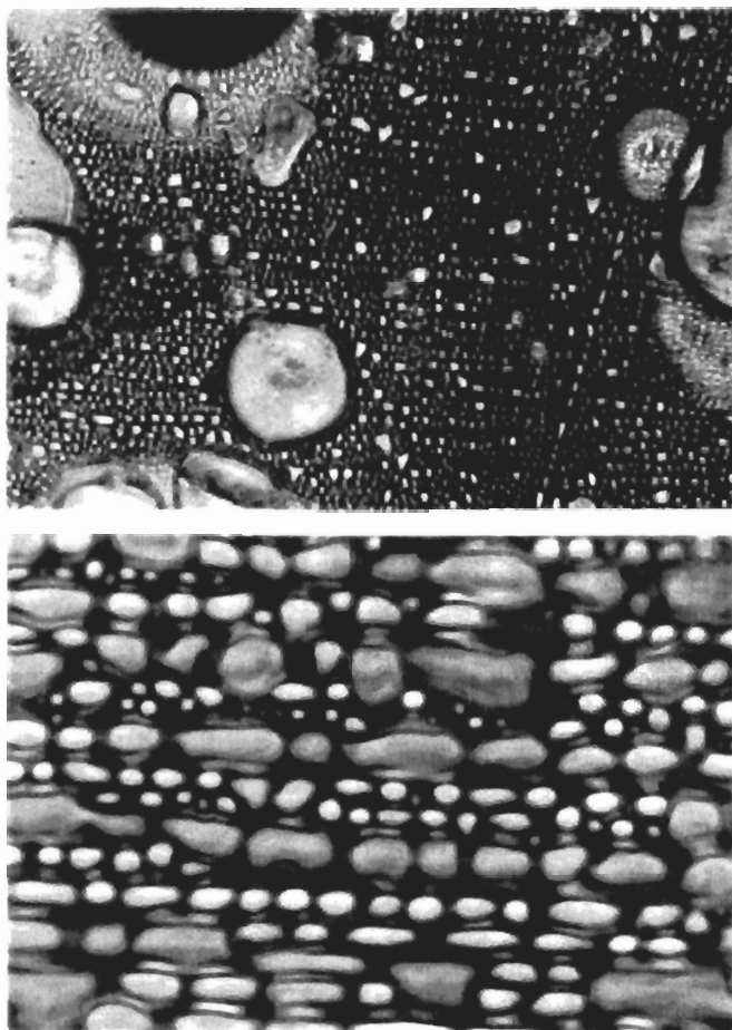
Figure 4.22. The top picture depicts under a 10× magnification a liquid magnecule composed of a bond between fragrance oil and water, the lower picture showing its 100× enlarged view. The pictures were obtained by the Givaudain-Roure Research Laboratories in Dubendorf, Switzerland. It should be indicated that the bubbles are partially fragrance oil and partially water, while the magnecule is the entire dark area of the pictures, which area was transparent water prior to Santilli's formation of the magnecular bond. Therefore, liquid magnecules may have specific weights of 10,000 amu or more, and are generally visible to the naked eye. It is instructive to know that tests at the same laboratory via an LC-MS conventionally set to identify oil fragrance molecules, showed no presence at all of any magnecular species because the analysts refused to use the largest available feeding line. In so doing, the analysts prohibited the admission in the LC-MS of the very species to be detected. This occurrence, rather frequent for analysts whose mind remains set at molecular detections, is confirmed by the fact that the LC-MS did detect the fragrance oil and water, but failed to provide any detection at all of the dark liquid of the pictures.
