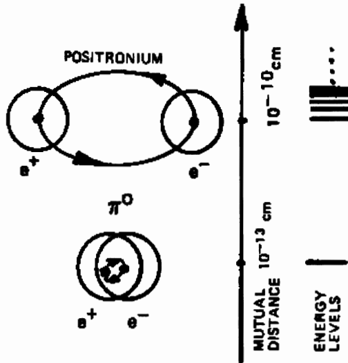
Figure 6.3. A reproduction of an original figure used by Santilli in 1978 to illustrate his model of the \pi^0 particle as "compressed positronium," namely, as consisting of one single additional bound state of the positronium under conditions of total mutual penetration of the constituents at 1 fm mutual distance verifying the covering hadronic mechanics. Santilli then showed that the model represents the totality of the characteristics of the \pi^0 , including rest energy, meanlife, charge radius, charge, spin, parity, magnetic moment and main decays.
