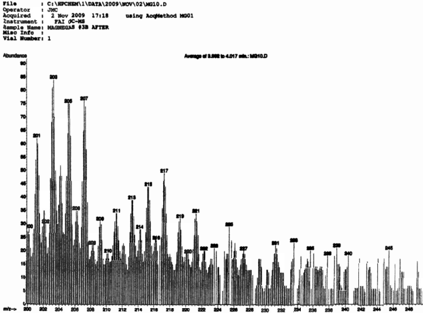
Figure 4.18. Yet another novelty of Santilli magneucle, the so called “accretion” of peaks by one amu that, evidently, can only be interpreted as the addition of one hydrogen atom, a new feature here illustrated from 200 to 250 amu, but which actually exist from 0 to 1,000 amu.
