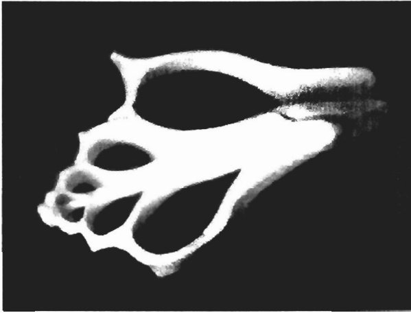
Figure 4.31. The slicing of a small seashell showing the various bifurcations despite its small size. The notion of time needed for a quantitative representation of the construction by the seashells of all these bifurcations is so complex to be truly beyond human comprehension. It can be represented via Santilli's hypertime consisting of the ordered set of four motions in future and past time, each one being multi-valued.
