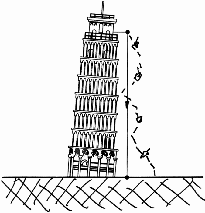
Figure 1.2. A schematic illustration of the tacit assumption in Galilei relativity of ignoring resisting forces in the free fall of massive bodies (here represented with the straight vertical line), as historically was the case in the celebrated experiments by Galileo Galilei in Pisa, while the actual trajectories within our atmosphere depart from such a behavior (here illustrated via the wiggly trajectory of a leaf in free fall in air).
