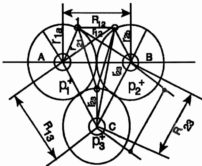
Figure 1.6. An illustration of the fact, actually proved by one of Santilli's graduate students, according to which the 20th century notion of valence in quantum chemistry predicts the capability of bonding hydrogen atoms into clusters H_n with an arbitrary number n of constituents, contrary to the evidence that the sole stable hydrogen molecule is H_2 . The occurrence is a direct consequence of the absence in the 20th century notion of valence of the restriction of the bond to individual pairs of valence electrons. Independently from all the above, identical electrons are predicted by quantum mechanics to repel and certainly not to attract each other, thus establishing truly fundamental insufficiencies in the most fundamental notion of 20th century quantum chemistry.
