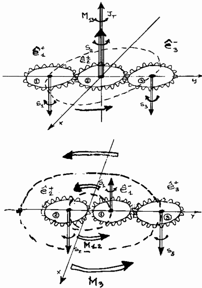
Figure 6.6. Reproduction of the original figure used by Santilli in Section 5 of the memoir 1978B to illustrate the dynamical differences between his structure model of the \mu^\pm (top view) and of the \pi^\pm (bottom view). In the former case, we have an isoelectron e^\pm at the center and two isoelectrons orbiting around, thus requiring no mutation of the angular momentum to represent the spin 1/2 of the muons. In the latter case, we have a \pi^0 at rest in the center (since it is much heavier than the electron) with an isoelectron e^\pm orbiting within the \pi^0 structure (since the size does not increase appreciably in the transition from the \pi^0 to the \pi^\pm ). In the latter case, a mutation of the total angular momentum of the isoelectron is necessary to represent the spin 0 of the \pi^\pm mesons. These two different values of the spin under the same number of elementary constituents are an excellent verification of the regular and irregular isorepresentations of the Lie-Santilli SU(2) spin symmetry outlined in the next section for the structure of the neutron. As we shall see, the two cases here considered are interpreted by Santilli as providing a direct distinction between electroweak and strong interactions (see HMMC Vol. III for details and references).
