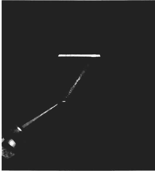
Figure 5.18. Light propagating within water constitutes visual experimental confirmation of Santilli's isorelativity due to the impossibility of quantitative representations via the reduction of light to photons scattered among water molecules, and the necessity of the local speed C = c/n as outlined in the text.
