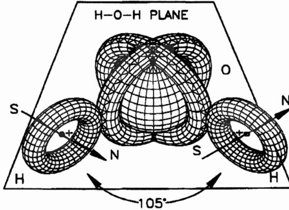
Figure 4.7. A view of the water molecule \text{H}_2\text{O} at absolute zero degree temperature, thus without any rotational degree of freedom, showing the \text{H}-\text{O}-\text{H} plane, the 105^\circ between the \text{H}-\text{O} and \text{O}-\text{H} dimers and, above all, the natural occurrence according to which the orbitals of the \text{H} atoms are not spherical, but of toroidal character for their coupling with the oxygen, thus providing a direct verification of the isochemical model of the hydrogen molecule of Figure 4.5.
