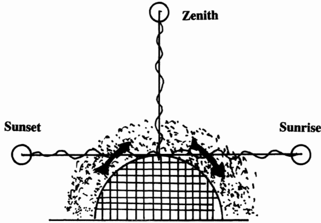
Figure 5.22. A schematic views by Santilli to illustrate the conventional Doppler redshift at Sunset and the conventional blueshift at Sunrise, as discussed in the text.
