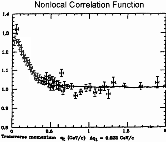
Figure 5.9. A reproduction of the excellent fit of the two-point isocorrelation function with experimental data on the Bose-Einstein correlation at very high energy from the celebrated UA1 experiments at CERN, first published by Santilli in 1991 ( loc. cit. ) and then re-examined by Cardone and Mignani in 1996 ( loc. cit. ). As one can see, the fit is a clear experimental verification of the validity of Santilli isorelativity in the interior of the proton-antiproton fireball. The fit reproduced in this figure may well result in being, in due time, the first experimental evidence on the ultimate nonlocality of the structure of the universe, with consequential needs for a suitable generalizations of contemporary local-differential mathematics, geometries, mechanics and relativities.
