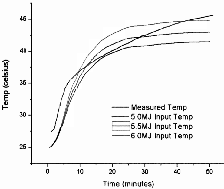
Figure 7.30. Thermal profiles of endplate.
