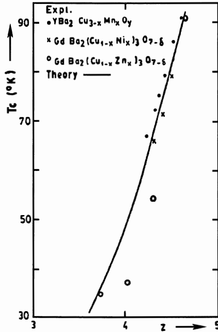
Figure 5.16. A reproduction of Fig. 5, p. 380 of Animalu [loc. cit.] showing the agreement between the prediction of isosuperconductivity for the doped 1:2:3 Cuprates and the experimental data.
