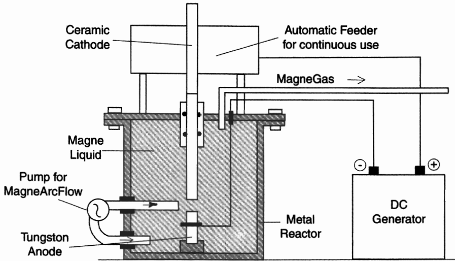
Figure 7.9. The main lines of Santilli hadronic refineries converting liquid waste into a clean burning, cost competitive gaseous fuel with magnecular structure, showing: the pressure metal vessel; the submerged electrodes; the recirculation of the feedstock through the arc; the external AC-DC converter; the external automatic controls of the arc; and the collection of the produced magnecular fuel.
