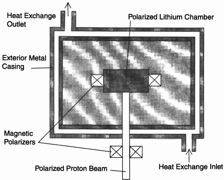
Figure 7.15. A schematic view of one of the simplest hadronic reactor, that for the synthesis of the lithium as per Eqs. (7.34).
