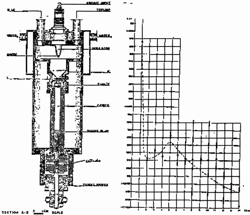
Figure 6.17. A view of Don Borghi's test equipment on the left and a typical activation curve on the right.
