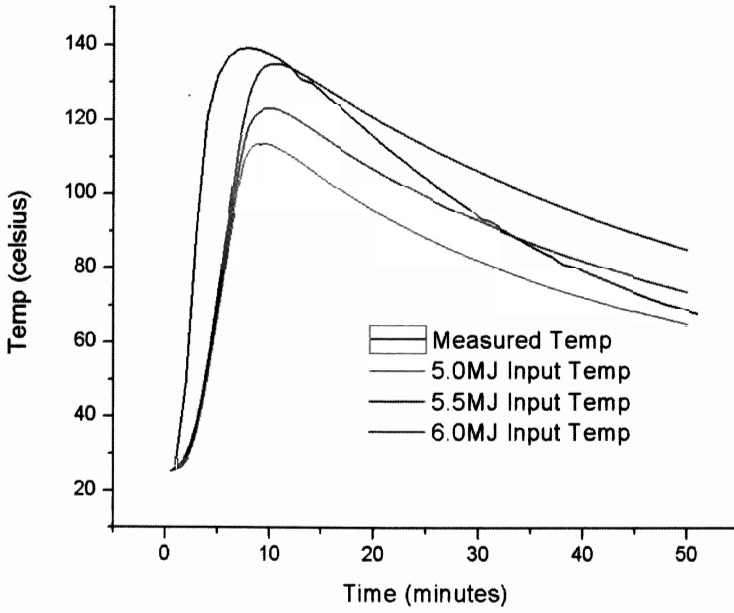
Figure 7.29. Thermal profiles of tube.
