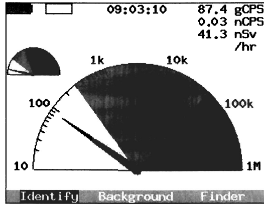
Figure 7.31. SAM940 Gamma and neutron detection.
