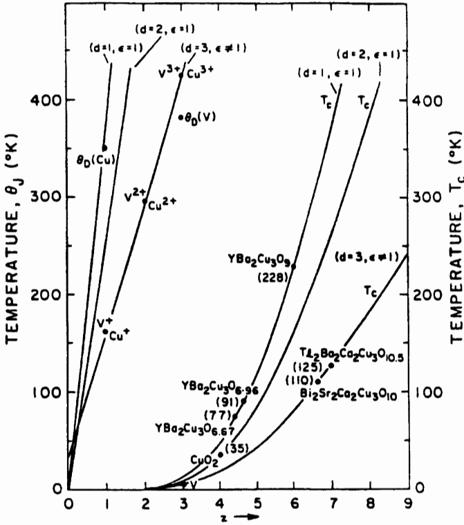
Figure 5.15. Animalu’s [loc. cit.] remarkable experimental verification of isosuperconductivity. The figure shows the plot between the theoretical prediction for the dependence of the superconducting temperature from the effective valence z of cuprate ions (continuous curve) and the experimental values on the “jellium temperature” for various compounds (solid dots).
