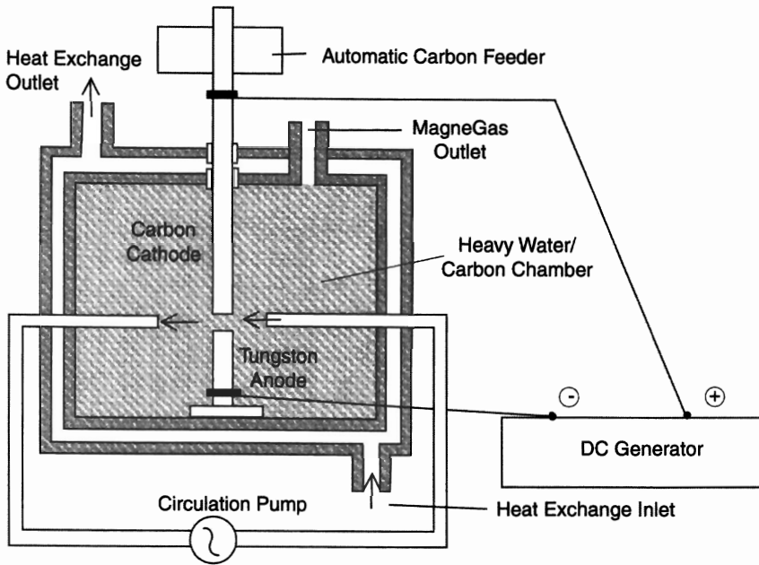
Figure 7.13. A schematic view of the Hadronic Reactor, essentially based on an engineering upgrade of the Hadronic Refineries of the preceding figures, showing the shift of emphasis, from the production and use of a magnequar fuel in the latter, to the production and use of heat in the former.
