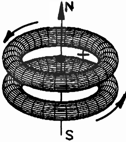
Figure 7.7. A reproduction of Figure 4.11 to illustrate the fundamental role of Santilli magneucleus for controlled nuclear fusion since they assure the correct spin coupling as per Law II.
