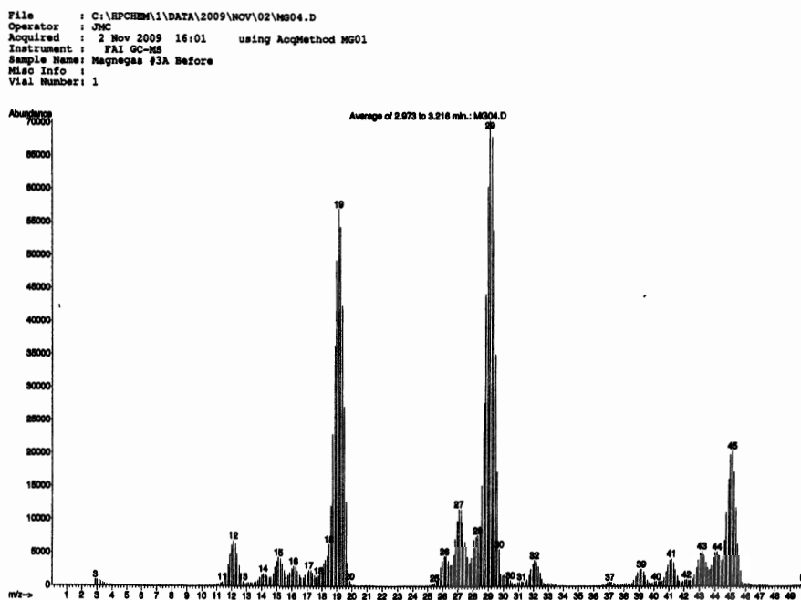
Figure 4.17. An additional illustration of the novelty of Santilli magneucle between 3 and 50 amu showing a peak at 19 amu now interpreted as H_3O = H - O - H \times H , another new peak at 29 amu interpreted as C - O \times H , and other peaks that can only be interpreted as being Santilli magneucle.
