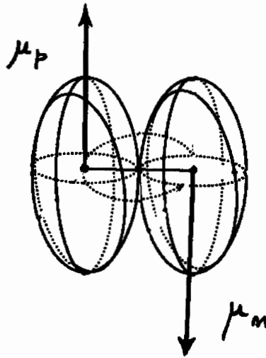
Figure 6.27. Reproduction of the figure used by Santilli to illustrate the impossibility by quantum mechanics to achieve an exact representation of the deuteron magnetic moment in a way compatible with the other characteristics such as total angular momentum, and charge radius.
