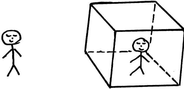
Figure 2.1. Santilli illustrates the far reaching implications of his isogeometries via the “isobox” consisting of a box inspected by two observers: an observer in the exterior verifying the conventional Minkowski spacetime, and an observer in the interior verifying the Minkowski-Santilli isospacetime. Santilli isonumbers and isospaces can be claimed to be understood if one understands that: the interior observer can be in the infinite future or past time with respect to the exterior observer; if the exterior observer sees a cube with 2-m side, the interior observer can see a room of dimension arbitrarily bigger or smaller compared to the exterior view; and if the exterior observer see a cube, the interior observer can see a cathedral. For explanations, interested readers should study the quoted literature.
