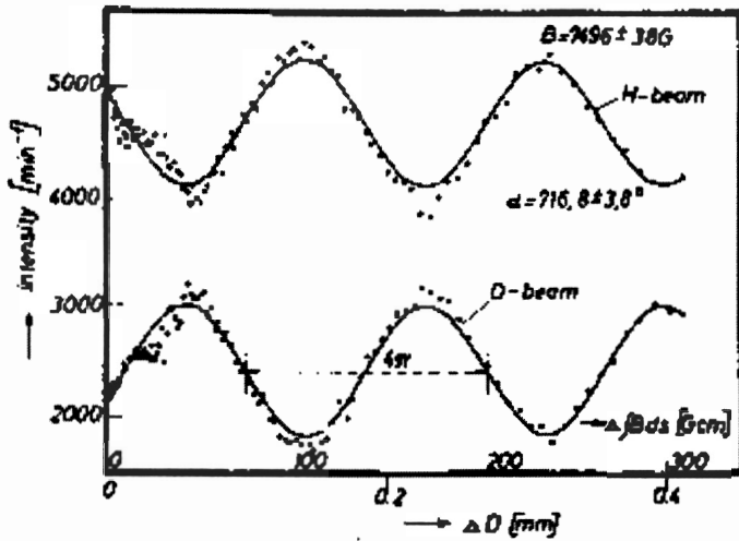
Figure 5.2. The plot of experimental data on the coherent recombination of the split neutron beams in Rauch's 4\pi neutron interferometric experiments of Figure 5.1. Note the loss of the sinusoidal character of the plot that, alone, establishes a deviation from the exact SU(2) -spin symmetry.
