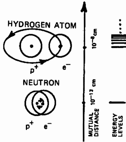
Figure 6.10. The sole bound state of a proton and an electron predicted by quantum mechanics is the hydrogen atom, with smallest orbit of the order of 10^{-8} cm. Thanks to the use of hadronic mechanics, Santilli has identified the existence of one and only one additional bound state, the neutron, characterized by the electron orbiting within the proton structure at distances of the order of 10^{-13} cm or less. Remarkably, Santilli has proved that the hadronic state is one and one only because, when excited, the isoelectron leaves the proton structure, thus recovering all conventional quantum states. In this sense, the energy levels of the hydrogen atom are the excited states of the neutron. As we shall see, these notions are at the foundation of the new hadronic energy studied in Chapter 7.
