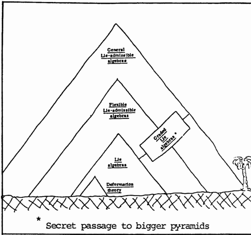
Figure 2.3. Another “vignette” presented by Santilli to his colleagues at the Lyman laboratory of physics of Harvard University at the initiation of his stay there in September 1978 under DOE support, illustrating the universality of Lie-admissible algebras because containing as particular cases all known or otherwise possible algebras. The study of Lie-admissible algebras encountered extreme opposition at Harvard University because of their consequential generalization of Einsteinian doctrines, quantum mechanics, quantum chromodynamics, and all that, as indeed achieved by hadronic mechanics thanks to Santilli’s resilience to academic vexations.
