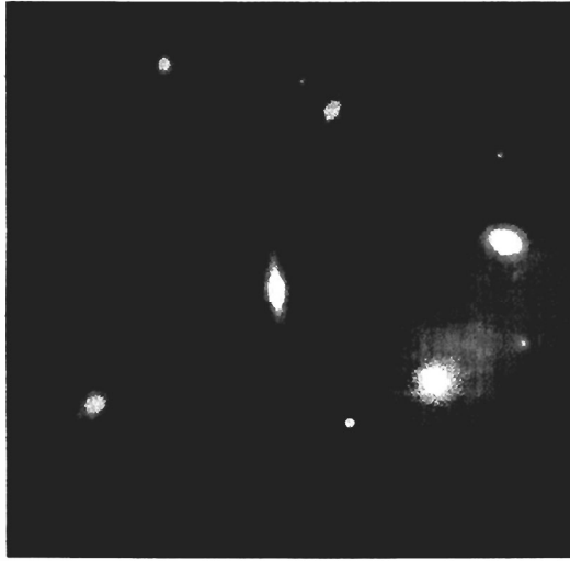
Figure 5.30. Santilli has defined “distressing” his studies of 20th century cosmology because of excessive assumptions, such as the expansion of the universe, “dark matter” and “dark energy,” intended to maintain the validity of Einsteinian theories under conditions they were not conceived, tested or intended for, rather than admitting their limitations, as well as the exclusion in cosmological models of biological structure and antimatter against the very Greek meaning of the word “cosmos.”
