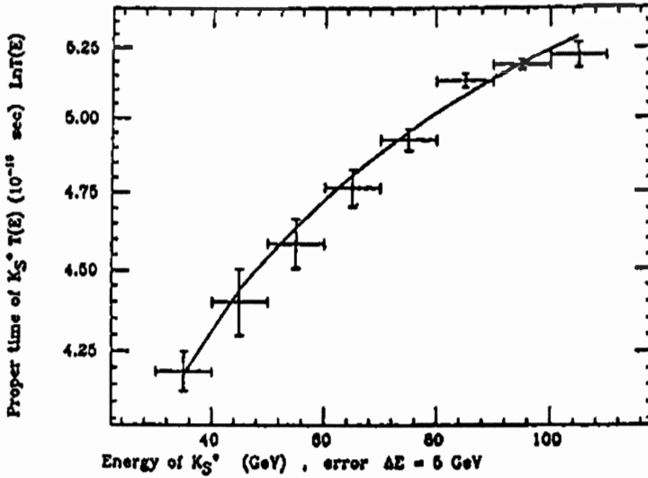
Figure 5.4. The exact plot done by Cardone et al. [75] (loc. cit.) of Aronson's experimental data (loc. cit.) via Santilli's isometric on the anomalous behavior of the meanlife of K^0 with speed in the energy range from 30 to 100 GeV.
