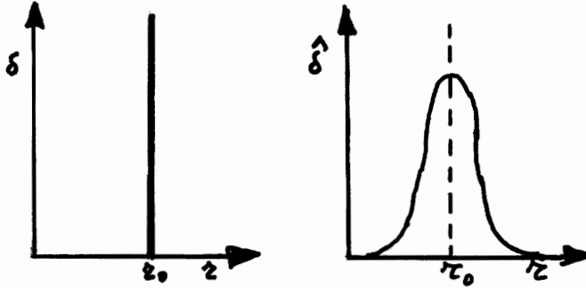
Figure 3.15. An illustration (left) of the origin of the divergencies of quantum mechanics in the singularity of Dirac’s delta function \delta(r - r_0) at the value r = r_0 , and their removal ab initio in hadronic mechanics (right) by the Dirac-Myung-Santilli isodelta function that no longer admits the preceding divergencies for a suitable selection of the isotopic element, here considered as being dependent on (r - r_0)^2 . In fact, the removal of the divergencies at the indicated level carries over at all levels the scattering and perturbation theories of hadronic mechanics.
