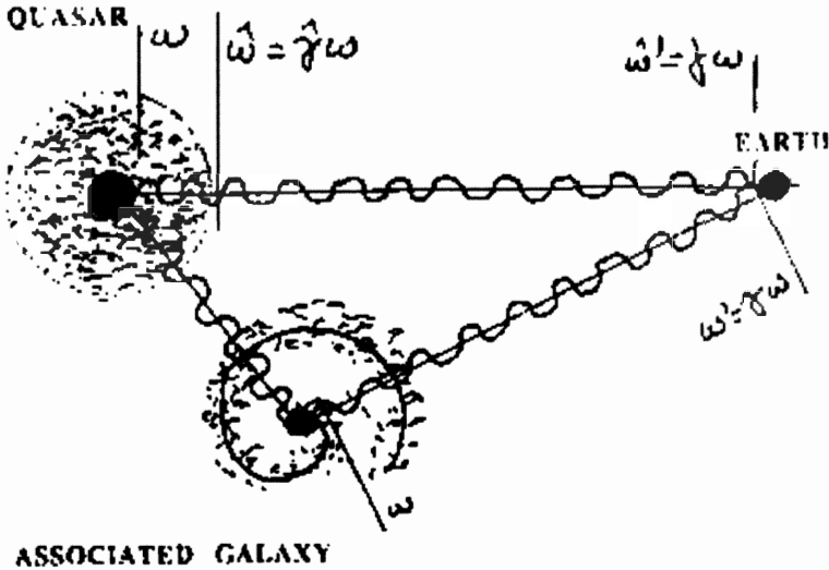
Figure 5.27. A reproduction of the original drawing by Santilli of 1988 illustrating the hypothesis on the isotopic origin of the quasar redshift, that is, a redshift due to the geometry of the huge quasars chromosphere. According to isorelativity, a first major component on the cosmological redshift of quasars is due to the decrease of the speed of light in its chromospheres. A second contribution is due to the anisotropy of the same medium. These two contributions then account for the complete difference in cosmological redshift between the quasars and the associated galaxy under the same relative speed v with respect to Earth.
