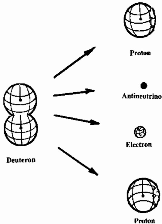
Figure 6.25. A reproduction of the drawing used by Santilli to illustrate the inability by quantum mechanics to represent the stability of the deuteron since the neutron is naturally unstable and, therefore, the deuteron should decay into two protons, an electron and the hypothetical antineutrino. No quantitative argument is known to the authors explaining the reason for the neutron to become stable when coupled to a proton. By comparison, Santilli's three body model of the deuteron represents its stability ab initio .
