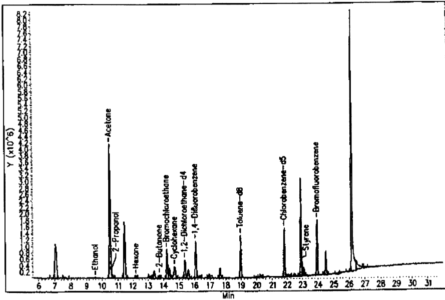
Figure 4.28. Experimental evidence of the magnecular structure of the HHO gas: a printout of the blank following completion of the scans with a GC-MS and removal of the gas from the instrument. For all conventional molecular gases, the blank solely shows background data none in macroscopic percentage. By contrast, the blank of this figure is essentially similar to the ordinary scan under the precautions indicated in Section 4.3 (sufficiently large feeding line, low column temperature, longest possible elusion time, etc.). Since the HHO gas was removed from the instrument, the above printout establishes the magnecular character of the gas via its anomalous adhesion to the walls of the instrument. Additionally, the scan shows a number of species in macroscopic percentage other than H_2 and O_2 that can only be explained as magnecular clusters comprising combinations of H or O, HO, H_2 , O_2 , and H_2O , since the gas originates from distilled water.
