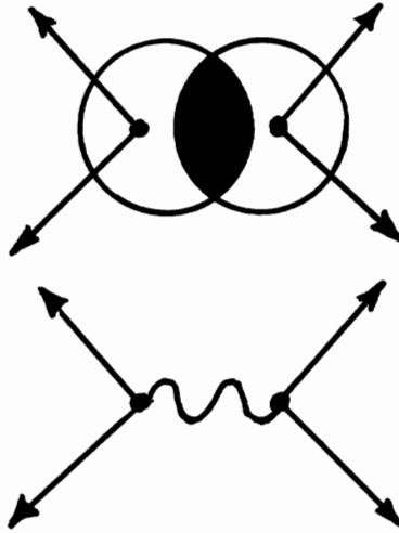
Figure 1.5. An illustration of the reason Santilli cannot accept the experimental data, let alone the basic theories, of the 20th century particle physics, illustrating the point-like abstraction of particles and their wavepackets (below), compared to the necessary deep overlapping of said wave-packets and/or charge distributions in high energy scattering experiments (above). Incontrovertible experimental evidence for deviations in scattering experiments from a point-like behavior establish the merely approximate character of the potential scattering theory and related lack of final character of the claimed “experimental results.” Additionally, Santilli cannot accept 20th century particle physics due to its irreconcilable incompatibility with other branches of physics, such as: incompatibility with Newtonian mechanics due to Theorem 1.1; incompatibility with thermodynamics due to the strict reversibility over time of particle physics compared with the irreversibility of thermodynamics; etc.
