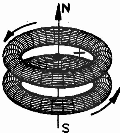
Figure 4.11. A conceptual rendering of an “elementary magneccule” comprising two identical or different atoms whose bond is entirely of magnecular character, namely, originating from opposing polarities North-South-North-South of the toroidal distributions of orbitals, as well as the polarization of nuclear and electron magnetic moments.
