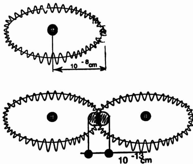
Figure 4.1. The original drawing used by Santilli to illustrate the physical differences between the hydrogen atom and the hydrogen molecule, the former consisting of point-like particles at large mutual distances, and the latter having additional short range interactions necessary for the valence bond. These physical differences illustrate the exact character of quantum mechanics for large mutual distances as in the hydrogen atom and its merely approximate character for additional short distance interactions as in the hydrogen molecule.
