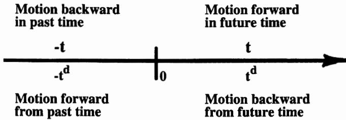
Figure 3.5. Contrary to popular beliefs, time has four directions as depicted by Santilli in this figure to illustrate the need for isoduality. In fact, time reversal can only allow the representation of two time directions. The remaining two time directions can solely be represented via the isodual map.
