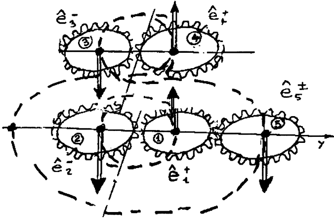
Figure 6.8. Reproduction of the original figure of memoir 1978B illustrating the structure model of the K^\pm with five constituents.
