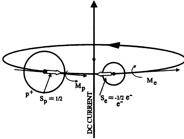
Figure 6.22. A schematic view of the geometry of a DC electric arc at subatomic distances in a ionized hydrogen gas. Note the alignment of polarized protons and electrons along the tangents to a magnetic line; a resulting axial coupling of protons and electrons under strongly attractive Coulomb forces due to opposite charges and magnetic polarities at short mutual distances; and the implausibility, under such a geometry, for protons and electrons to acquire 0.782 MeV relative kinetic energy “to fix things” in favor of preferred doctrines [102, 103].
