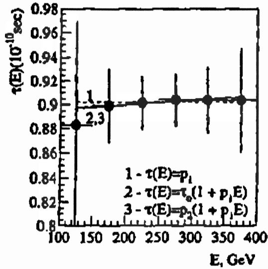
Figure 5.6. A view of three plots made by Arestov et al. (loc. cit.) via the use of Grossman’s statistics of tests (loc. cit.) on the energy dependence of the meanlife of the neutral kaon on the energy showing the dominance of the PC violation selected in Grossman’s tests to such an extent to show an apparent lack of dependence of the meanlife on energy, while the same dependence is clear in the different parametrization selected in the data elaborations by Aronson (loc. cit.) as well as Aronson (loc. cit.). These and numerous other equivocal aspect cast serious shadows on the acceptance for publication of the paper by Grossman’s et al. without a more serious scrutiny.
