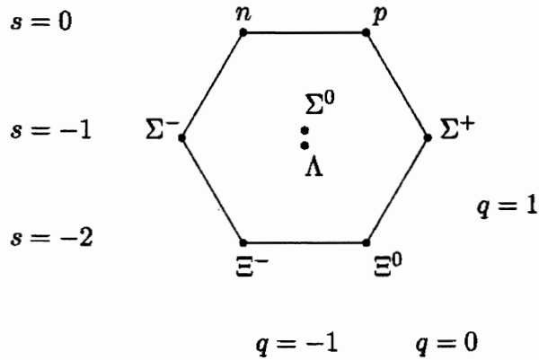
Figure 6.14. A view of the well known octet of baryons (from Wikipedia).
