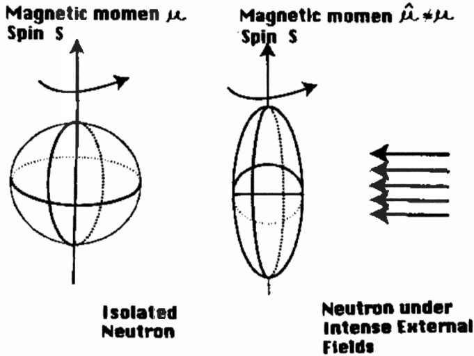
Figure 5.3. The elementary physical interpretation of Rauch’s measurements of Figures 5.1 and 5.2 via a deformation of the charge distribution of neutron of the order of 1%. Note that the deformation must be such as to provide an oblate spheroidal ellipsoid as a condition to represent the “angle slow down effect,” since only such oblate deformation implies a decrease of the intrinsic magnetic moment. Note also that the spin 1/2 of the neutron is not mutated in Rauch’s experiment due to the external long range nature of the electric and magnetic fields acting on the neutron and the absence of contact interactions. The preservation of the spin 1/2 implies that quantitative treatments can be obtained via nonunitary transforms of conventional relativistic treatments, technically expressed by the fact that the irreducible representation of the Lorentz-Poincaré-Santilli isosymmetry are regular (the “exceptional representations” implying an alteration of the spin that cannot be obtained via such a simple map).
