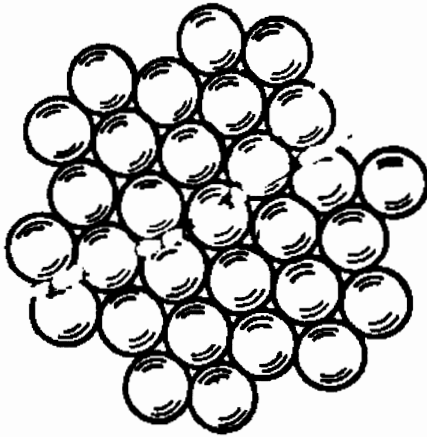
Figure 7.5. A reproduction of Figure 6.24 often used by Santilli to illustrate that “nuclei have no nuclei” being composed by extended constituents in contact with each other (technically, in conditions of mutual penetration of about 10^{-3} of their charge distributions). Consequently, the nuclear force is expected to be partially of potential and partially of nonpotential type, with ensuing nonunitary character of the theory, and related applicability of hadronic mechanics.
