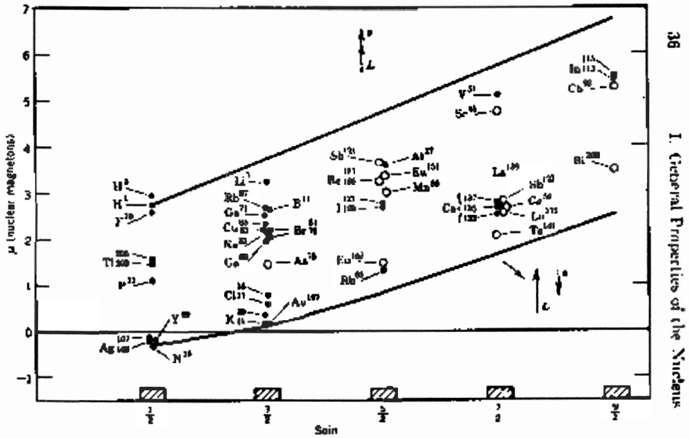
Figure 5.12. Additional evidence of the lack of exact character of quantum mechanics in nuclear physics given by experimental data on nuclear magnetic moments that do not follow quantum predictions, and are instead comprised between certain maximal and minimal values partly reproduced in this figure from known nuclear sources.
