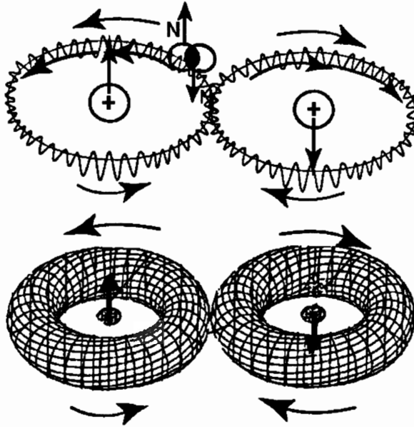
Figure 4.4. A view of isochemical model of the hydrogen molecule at absolute zero degrees temperature, thus without any rotational degree of freedom, with the Santilli-Shillady strong valence bond between valence electrons pairs into the isoelectronium quasiparticle. Note the o-shaped orbital of the isoelectronium, the only one allowing a representation of the diamagnetic character since, under an external strong magnetic field, the two H atoms acquire parallel but opposite magnetic polarities with null value at sufficient distance. Note also the toroidal distribution of the orbital of the isoelectronium due to the isouncertainty principle of hadronic mechanics.
