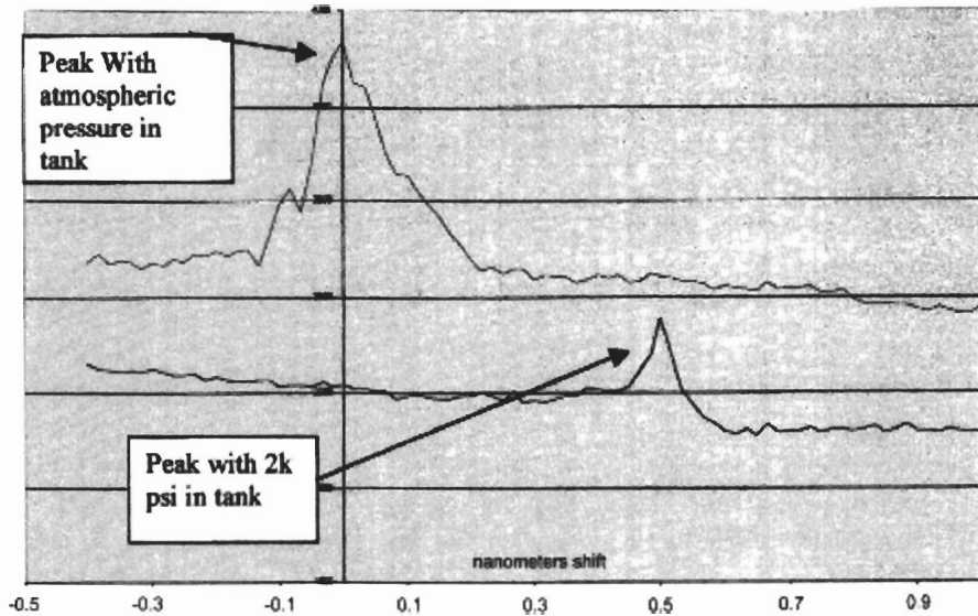
Figure 5.20. A view of the first detection of Santilli's isoredshift obtained in June 27, 2009, at the Isoredshift Testing Station of the preceding figure showing a clear increase of the wavelength with consequential clear decrease of the frequency of the used blue laser light. Additional pictures and data are available from the website http://www.santilli-foundation.org/Sunset-Sunrise.html (Inconsistencies of special relativity within physical media, R. Anderson, The R.M. Santilli Foundation).
