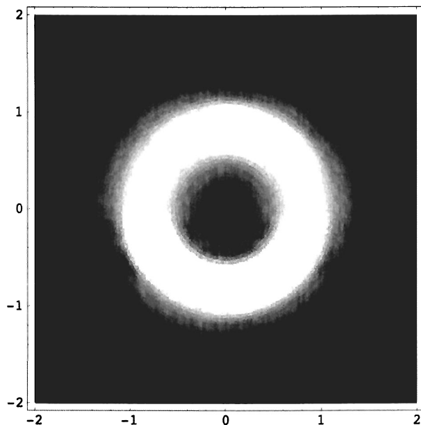
Figure 4.9. The new chemical species of Santilli magnecules requires an atomic technology capable of polarizing the orbitals of individual atoms (rather than molecules) into a toroidal form (rendering by A. K. Aringazin).
