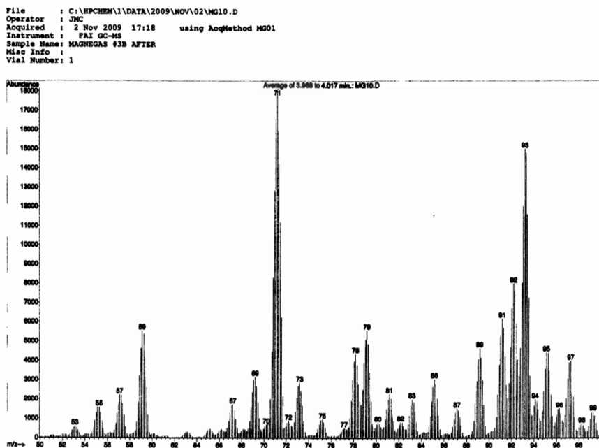
Figure 4.16. A more detailed view between 50 to 100 amu of the preceding FAI scan.
