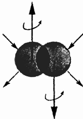
Figure 4.2. A reproduction of the original picture used by Santilli on the valence electrons bond in single coupling illustrating the need for a theory that is nonlinear (in the wavefunction), non-local (of integral type) and nonunitary (because of contact nonpotential type not representable with a Hamiltonian). Quantum chemistry is strictly linear, local-differential and Hamiltonian, thus being structurally unable to provide a quantitative representation of the valence. By comparison, the covering hadronic chemistry has the needed nonlinear, nonlocal and nonunitary structure beginning with its mathematical foundation.
