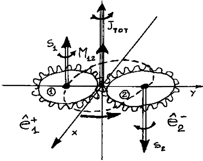
Figure 6.5. A reproduction of Fig. 2, page 852, of memoir 1978B depicting the “gear model” used to illustrate the general law of hadronic mechanics according to which, when in conditions of mutual penetration of the wavepackets and/or of the charge distributions, only singlet couplings of spinning particles are stable, while triplet couplings are highly unstable. In fact, gears can only be coupled in singlet, as shown in the figure, while their triplet coupling implies high repulsive forces. Note that this law does not exist for quantum mechanics since the particles in this case are dimensionless points, thus allowing both singlet and triplet couplings.
