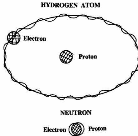
Figure 6.1. An original drawing used by Santilli in his lectures to illustrate the dramatic physical differences between the hydrogen atom and the neutron synthesis from a proton and an electron as occurring in stars. In the former case, the large mutual distance allows an effective point-like abstraction of the proton and the electron, resulting in the exact validity of quantum mechanics. In the latter case, the use of the same abstraction causes the exiting from the boundary of science in favor of theologies due to the condition of total penetration of the electron within the hyperdense medium inside the proton, with the resulting inapplicability of quantum mechanics due to the emergence of contact non-Hamiltonian forces that are basically absent in the hydrogen structure.
