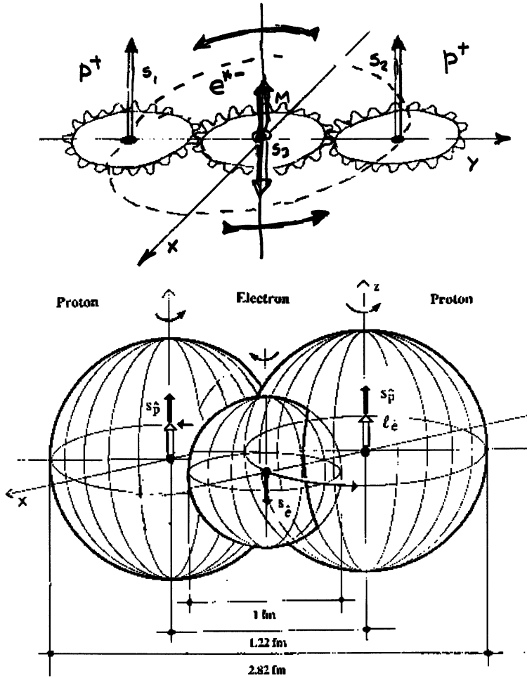
Figure 6.28. Reproduction of two original drawings used by Santilli to illustrate his conception of the structure of the deuteron as a restricted three body of two un-mutated protons (due to their weight) and one mutated electron. As reviewed in detail in the following sections, the top view uses the very effective “gear model” to avoid the highly repulsive triplet couplings, while the bottom view is the same as the top view, the particles being represented with overlapping spheres.
