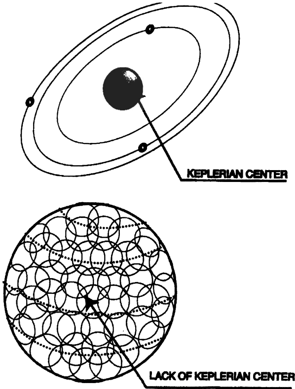
Figure 5.11. A visual evidence of the impossibility for quantum mechanics to be exactly valid in nuclear physics voiced by Santilli in numerous of his writings: the fact that “nuclei do not have nuclei,” thus causing the breaking of the fundamental Galilean and Lorentz-Poincaré symmetries of quantum mechanics (see also Figure 1.2). The impossibility for quantum mechanics as being exact for the nuclear structure is then beyond credible doubt.
