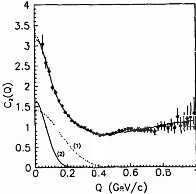
Figure 5.10. Another exact fit of the experimental data on the Bose-Einstein correlation for proton and antiproton annihilation, this time, at low energy. Curves indicated with 1 and 2 represent the fits with quantum models. Their dramatic deviation from experimental data is sufficient to disqualify any claim on the exact validity of quantum mechanics for the Bose-Einstein correlation that, unfortunately, has been rather widespread during the physics of the second half of the 20th century.
