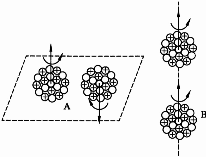
Figure 7.6. A schematic view of the only two stable couplings permitted by hadronic mechanics for nuclear fusions, the “singlet planar coupling” of the l.h.s. and the “triplet axial coupling” of the r.h.s. All other spin configurations have been proved to produce strongly “repulsive” forces under which no CNF is systematically possible.
