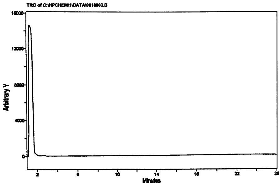
Figure 4.14. Following the failure by the computer to identify any of the detected peaks, Santilli requested the analysts to inspect the same peaks under the IRD. The above figure established that none of the peaks in the mass spectrum between 40 amu and 400 amu had any IR signature at all, thus establishing the the bond of the peaks cannot possibly be of valence type, since the sole molecule that shows no IR signature is the hydrogen and a few others light with orbitals having perfect spherical symmetry. The appearance in the computer screen of the IR scan of this figure has potentially historical meaning because it constitutes clear experimental evidence of the novelty of the bond. In fact, the analysts showed great surprise at the view of this scan and indicated to Santilli that he had indeed discovered a “new chemical species” which could not be that characterized by valence bonds. The analysts of the McClellan Air Force Basis then released a signed statement of novelty reproduced in the historical 1998 paper as well as in FHC.
