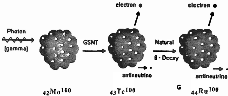
Figure 7.35. A schematic view of the example of hadronic fuel proposed by Santilli in his 1994 paper, the isotope of molybdenum Mo(100, 42, 0). Note that all other Molybdenum isotopes were proved not to admit a stimulated beta decay. Note also that quantum mechanics does predict the double beta decay, but with very small amplitude, thus being of no practical value. Stimulated double decay in appreciable percentage are solely predicted by hadronic mechanics and specifically when using photons with a specific resonating frequency never studied via quantum mechanics.
