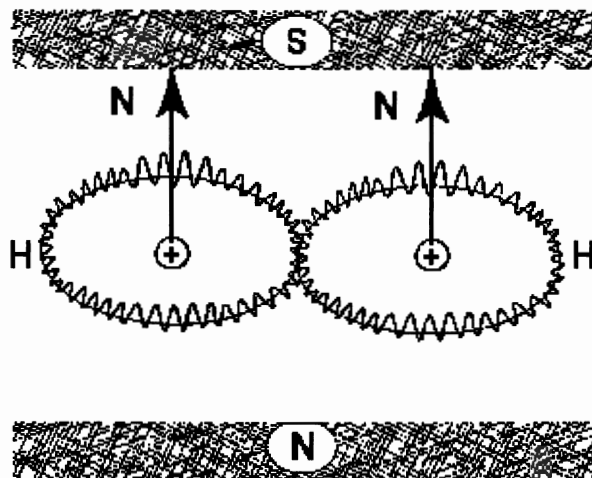
Figure 4.3. The original drawing used by Santilli to illustrate a catastrophic consequence of the quantum chemical notion of valence, the prediction of the paramagnetic character of all substances. The prediction includes the hydrogen molecule, in dramatic disagreement with experimental evidence according to which the hydrogen molecule is diamagnetic, thus being unable to acquire a total magnetic polarization under an external magnetic field. The indicated prediction is a consequence of the absence in quantum chemistry of a strongly attractive valence force, in which case valence electrons are unconstrained and, consequently, can acquire independent magnetic polarizations under an external magnetic field. The picture provides a conceptual rendering of the two H-atoms of the hydrogen molecule as essentially being independent. The alternative conception of orbitals distributed around the two nuclei carries an even stronger prediction of paramagnetic character because it can acquire more easily a total polarization under an external magnetic field contrary to nature.
