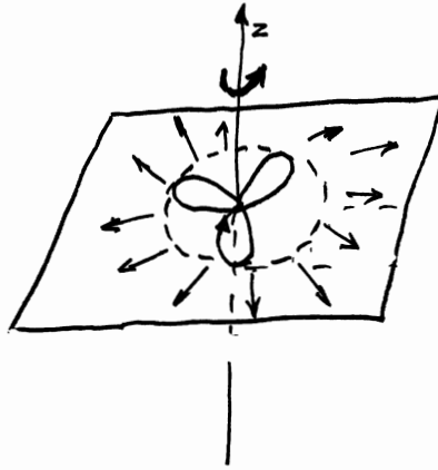
Figure 3.1. An original drawing by Santilli dating back to 1955 on his conception of the structure of the electron as a pure oscillation of a point of the ether, showing the distribution on a plane due to rotation, the longitudinal force propagated through space, thus being interpreted as the origin of the electric charge, Eq. (3.2).
