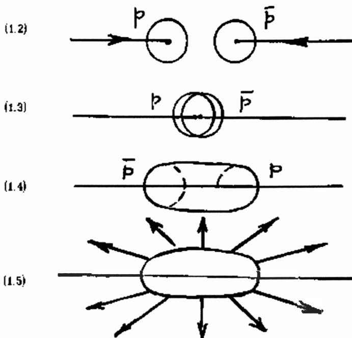
Figure 5.8. A schematic view of the Bose-Einstein correlation originating in proton-antiproton annihilations. The top view depicts the event as permitted by quantum mechanics, that is, with the necessary abstraction of protons and antiprotons as massive points, in which case no correlation is conceptually or technically possible (see the text). The lower views depict the event as described by the covering hadronic mechanics, according to which the proton and the antiproton are represented with their actual, extended, non-spherical and deformable shape. The particles first coalesce, then they annihilate and form the so-called "fireball," namely, a spheroid ellipsoid whose prolate character depends on the energy of the particles. The fireball then decays into numerous unstable hadrons whose final product is given by correlated mesons released in all space directions.
