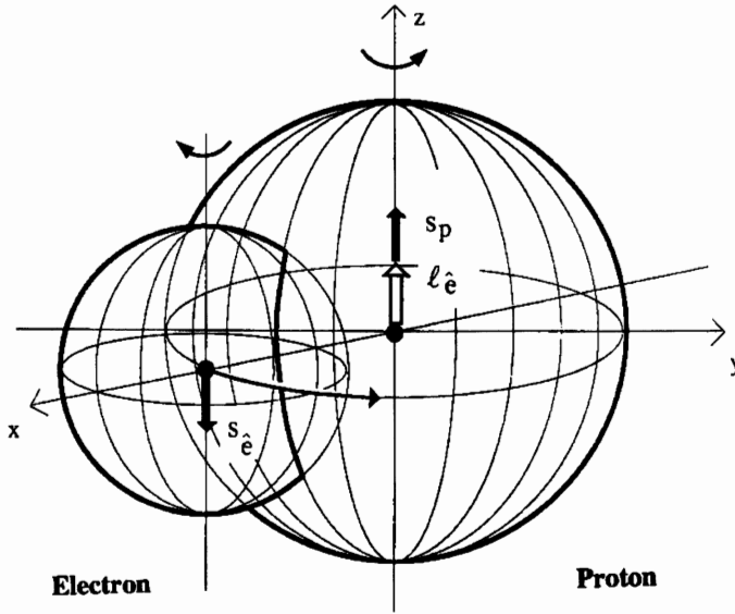
Figure 6.11. A reproduction of Figure 1 of Santilli 1990 on the spin of the neutron as permitted by hadronic mechanics. The main feature is the abandonment of the abstraction of the proton either as a point, or as a sphere with isolated points in its interior, as necessary for the applicability of quantum mechanics, and the representation of the proton as it is in the physical reality, a sphere of about 1 F in radius containing one of the densest media measured in laboratory until now. Then, at the initiation of “Rutherford’s compression” of the electron inside such hyperdense medium, it is evident that the electron is captured and constrained to rotate around the proton with an angular velocity equal to the proton spin. But the electron and proton can only couple in singlet for stability. It then follows that the total angular momentum of the isoelectron is null and the spin of the neutron coincides with the spin of the proton.
