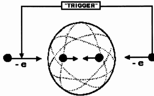
Figure 6.4. A conceptual rendering of Santilli’s “trigger” consisting of an external action (such as collision, pressure, etc.) forcing particles to pass through the “hadronic horizon” (the sphere of radius 1 fm) with consequential activation of strongly attractive forces discussed in the text.
