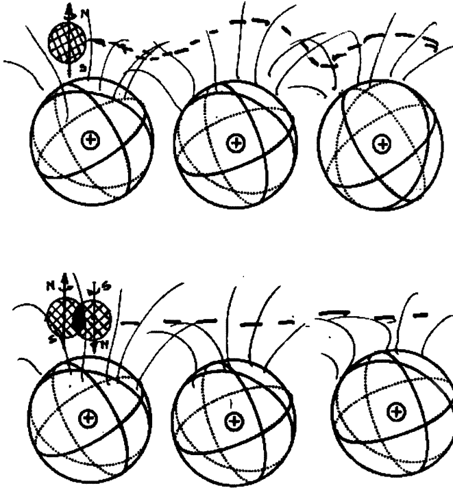
Figure 5.14. A schematic view of a conventional current of individual electrons (top view) and a superconducting current of Cooper pairs (lower view). The smaller electric resistance experienced by the latter as compared to that of the former current is due to the absence in the Cooper pair of an appreciable magnetic moment from its singlet structure, resulting in much smaller interactions with the atoms of the conductor. Note that we are here referring to a basically new current not yet industrially realized.
