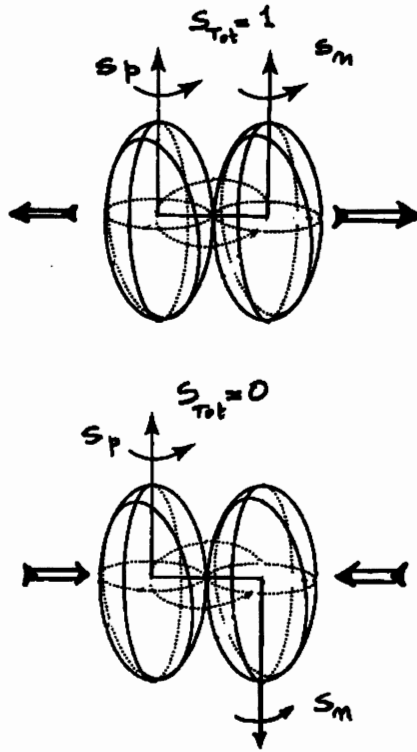
Figure 6.26. Reproduction of the original drawing used by Santilli to illustrate the impossibility of quantum mechanics to represent the spin 1 of the deuteron in a way compatible with its size. In fact, spin 1 can solely be achieved with a triplet coupling (top view), in which case no stable nucleus is conceivable due to very strong repulsive forces at the distance of nuclear forces. The only stable state is the singlet (bottom view), but in this case the total angular momentum is zero, in disagreement with experimental evidence.
