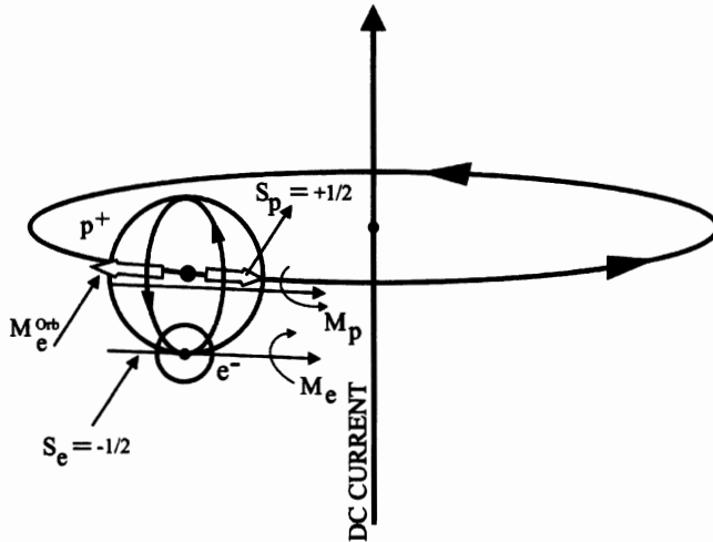
Figure 6.23. The inevitable bond of the polarized proton and electron of the preceding figure due to strongly attractive coulomb interactions for opposite charges and magnetic moments, presented by Santilli as a realization of Rutherford's "compressed hydrogen atom." Note that, at this stage, the particle has the charge and dimension of the neutron, but not its rest energy, spin and magnetic moment, thus being intermediate prior to the full synthesis of the neutron, the latter occurring under a sufficient external "trigger."
