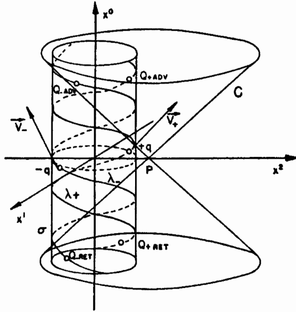
Figure 3.4. A schematic view of the calculations via advanced and retarded field theoretical methods, used by Santilli in 1974 to establish the incompatibility of Einstein's gravitation with quantum electrodynamics, in this case showing the entire electromagnetic origin of the exterior gravitational mass of the \pi^0 particle, in irreconcilable disagreement with the null source of Einstein's field equations for the case considered.
