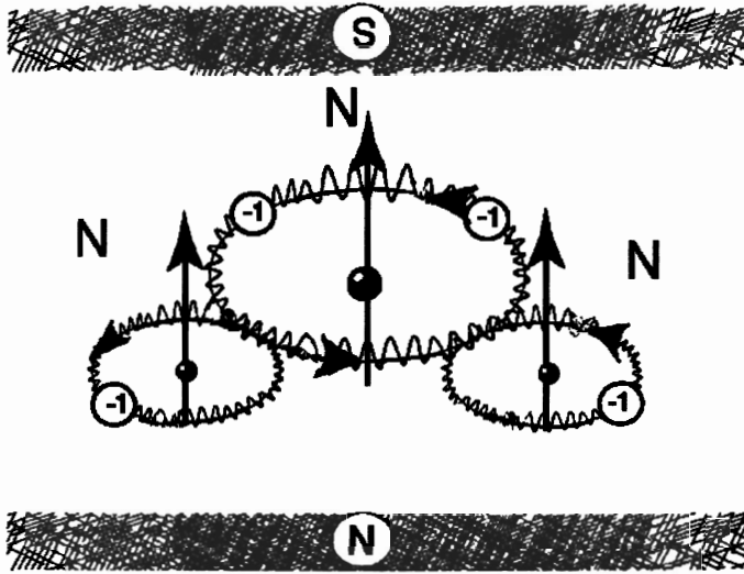
Figure 1.7. A view used by Santilli to illustrate the prediction by quantum chemistry that all substances, such as water, are paramagnetic, in dramatic disagreement with evidence. The prediction is a consequence of the lack of a “strongly” attractive force between valence electron “pairs,” as occurring in nature, in which absence valence electrons remain essentially independent, thus capable of acquiring a magnetic polarization, of course, under a sufficiently strong external magnetic field.
