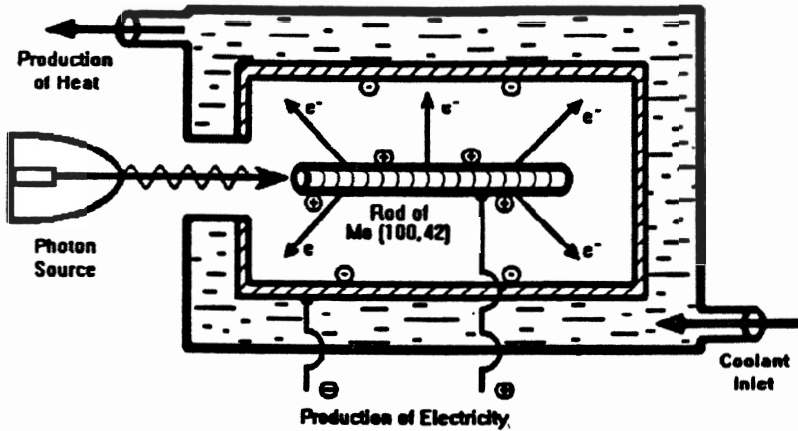
Figure 7.36. A schematic view of the hadronic reactor proposed in the 1994 paper consisting of: a coherent beam of resonating photons hits a bar of Mo(100, 42) with the stimulated transmutation into Tc(100, 43) with the emission of a first highly energetic electron, followed by the spontaneous decay of Tc(100, 43) into Ru(100, 44) with the emission of a second highly energetic electron. The electrons are captured by a metal shield that absorbs also the energy corresponding to the decrease in mass from Mo(100, 42) to Ru(100, 44). Additionally, the difference in potential between Mo(100, 42, 0) and the shield produces a DC current.
