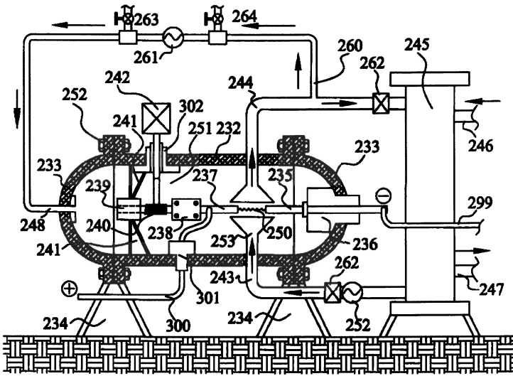
Figure 7.14. A more detailed view of a preferred embodiment for the industrial realization of hadronic reactors proposed for the industrial realization of ICNF.
