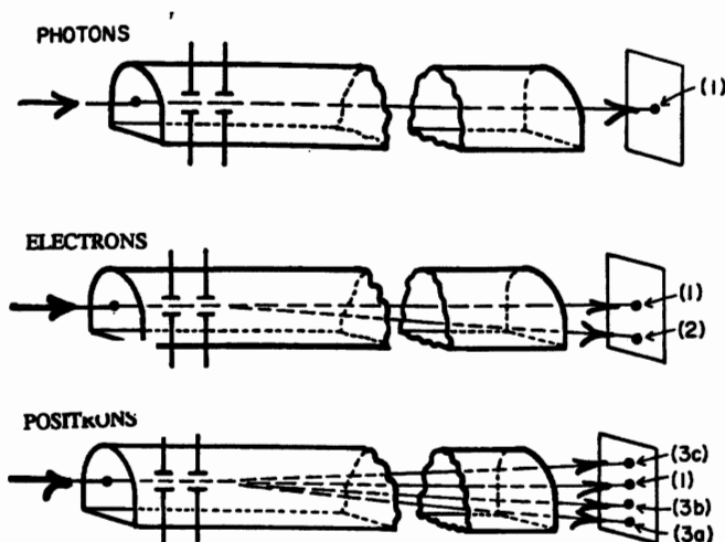
Figure 3.6. The original illustration used by Santilli for the 1994 proposal to test the gravity of positrons in horizontal flight in a vacuum tube. The proposal has been qualified by experimentalists as being technically feasible nowadays and resolutive because the displacement due to gravity on a scintillator at the end of a 10 m flight for positrons with milli-eV energy is visible to the naked eye. The usual criticisms based on disturbances caused by stray fields have been disqualified as political for a tube with at least 50 cm diameter. Virtually all major physics laboratories around the world have rejected even the consideration of the test, despite its dramatically lower cost and superior scientific relevance compared to preferred tests, on grounds that “Einstein theories do not admit antigravity,” although with documented knowledge that said theories cannot consistently represent antimatter as reviewed in the test.
