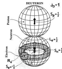
Fig. 12: A view of the structure of the Deuteron according to the synthesis of the neutron from a proton and an electron in the core of Stars ([83] and Appendix B).
